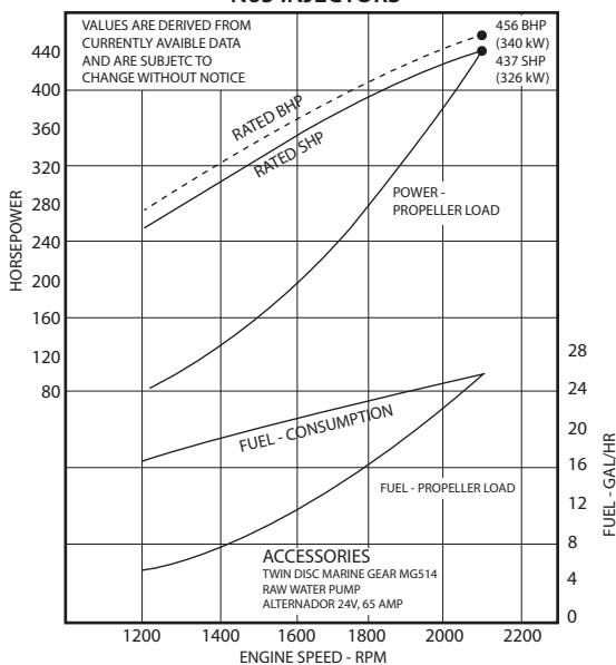
MODEL 12V-71 MARINE INTERMITTENT RATING N65 INJECTORS
